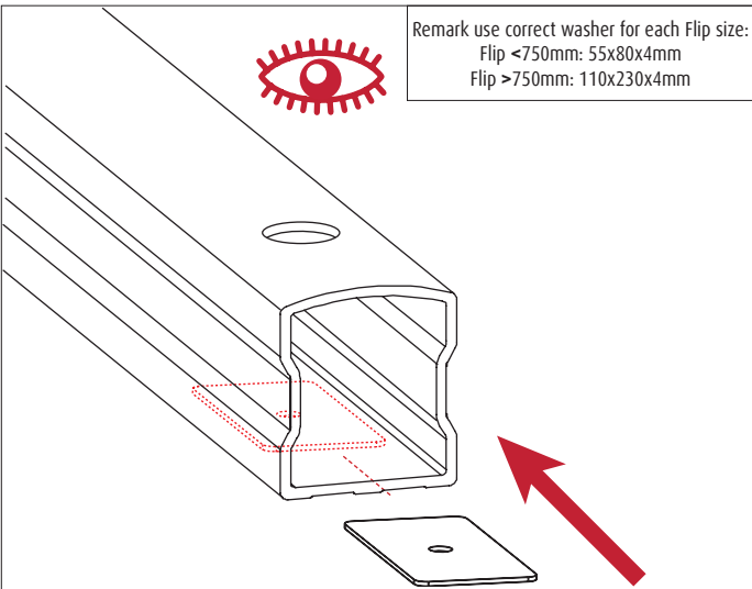
9 Place a washer trough the sides and position correctly
