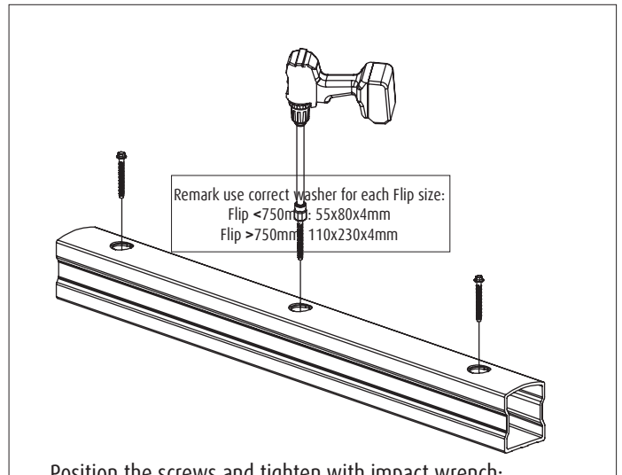
10 Position the screws and tighten with impact wrench; Torque = 100 Nm
