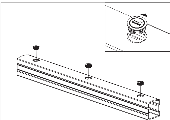
9 Place a washer trough each hole and position correctly
