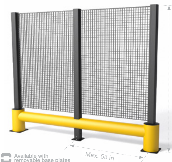
TB 400 PLUS FENCE 20.10 kJ
